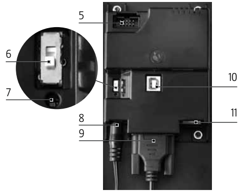
MDB interface (in behuizing)
